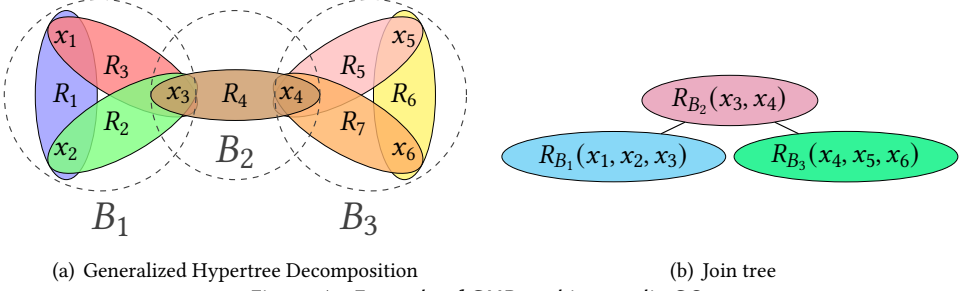
Fig. 3. An Example of GHD and its acyclic CQ.
