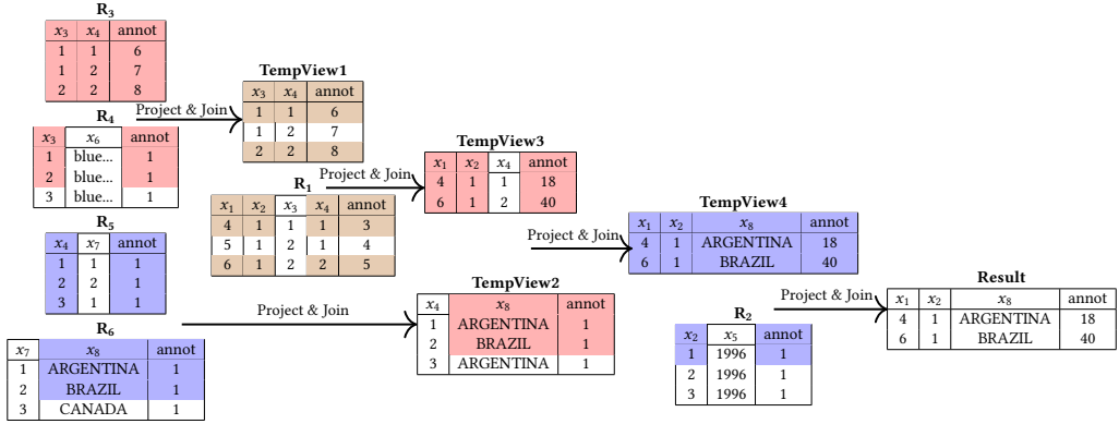
Fig. 13. A running example of Example 2.1
