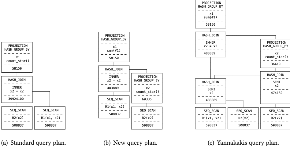
Fig. 14. Query plans for Q_4 in DuckDB.
