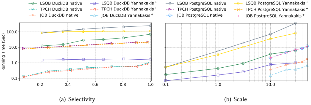
Fig. 11. Running times of different selectivity & scale.
