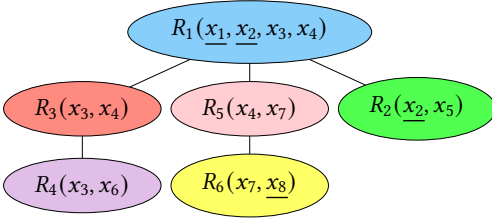
Fig. 5. Join tree \mathcal{T}_3 for Q_1 .
