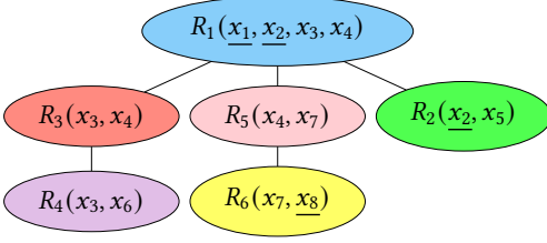
Fig. 5. Join tree T_3 for Q_1 .
