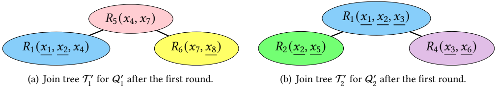
Fig. 2. Two Jointrees for Q'_1 and Q'_2 .
