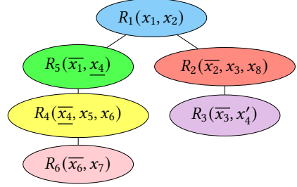
Fig. 6. Join tree for Q'_5 .
